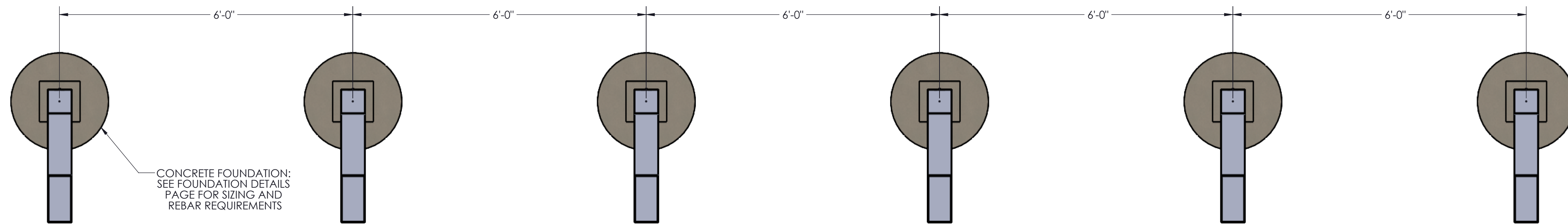
TOP VIEW LAYOUT FOOTING & BLOCKOUT
