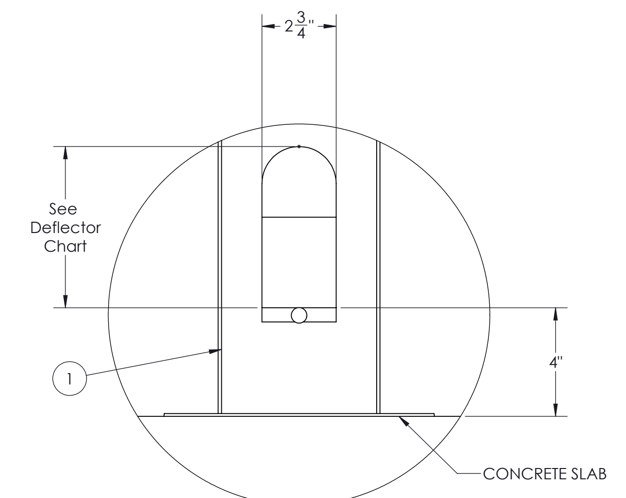
COLUMN DRAIN HOLE DETAIL SCALE 1:3.5
