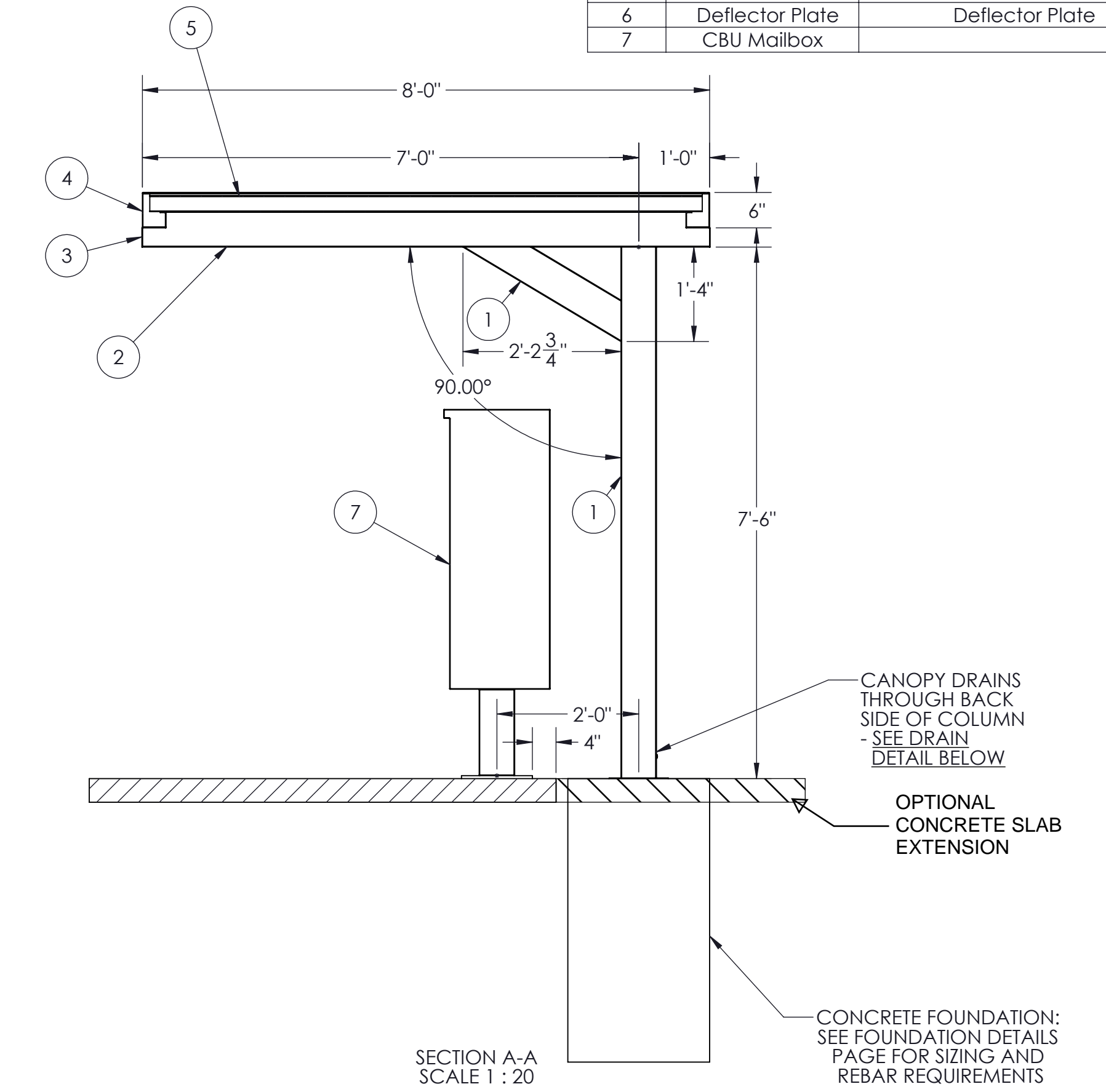
SECTION VIEW
