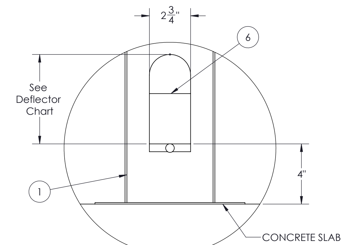
COLUMN DRAIN HOLE DETAIL SCALE 1 : 4
