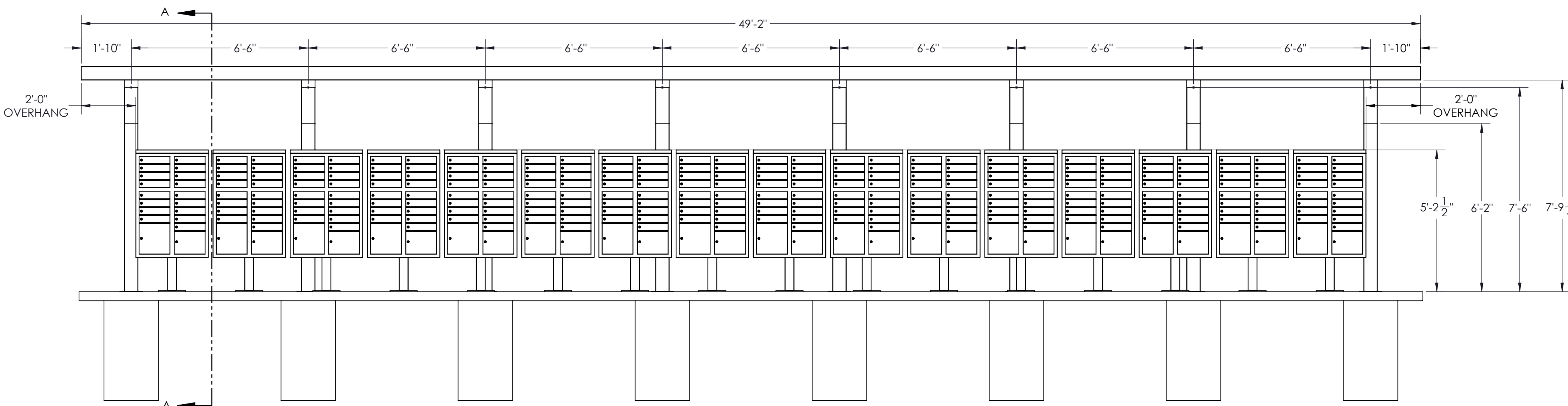
ELEVATION VIEW
