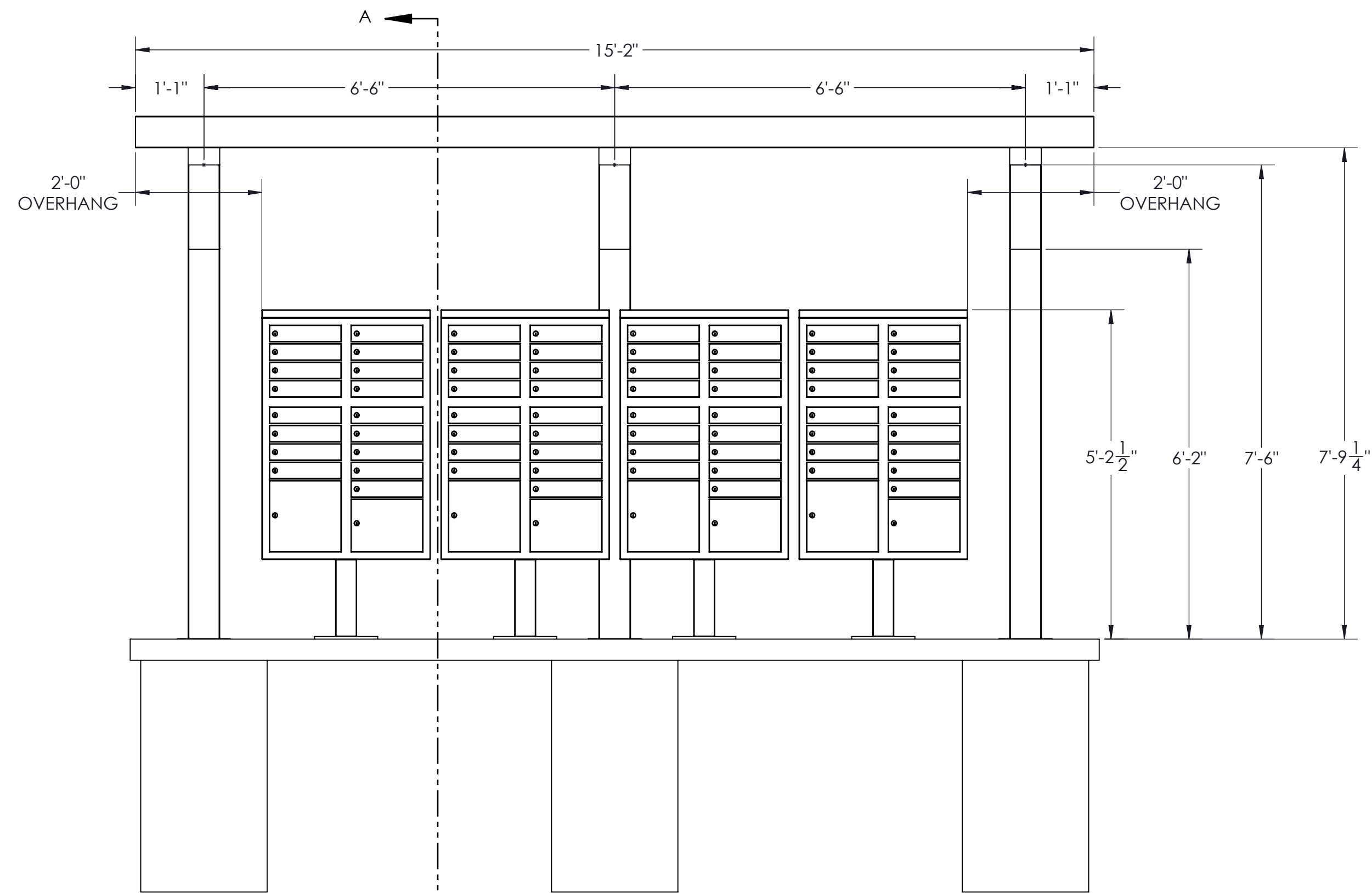
ELEVATION VIEW
