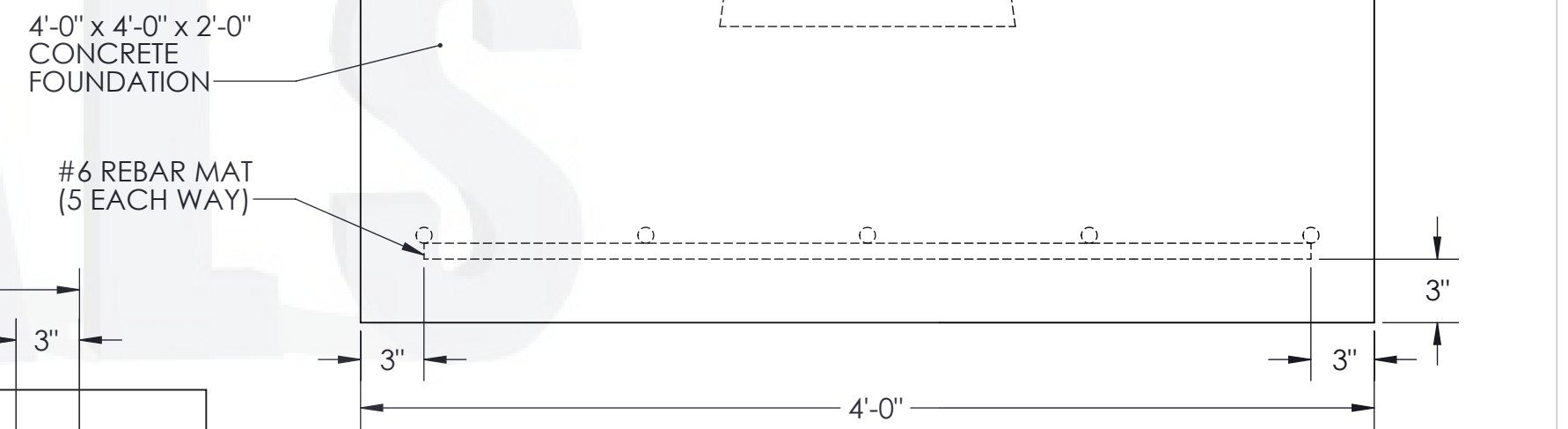
SIDE VIEW
