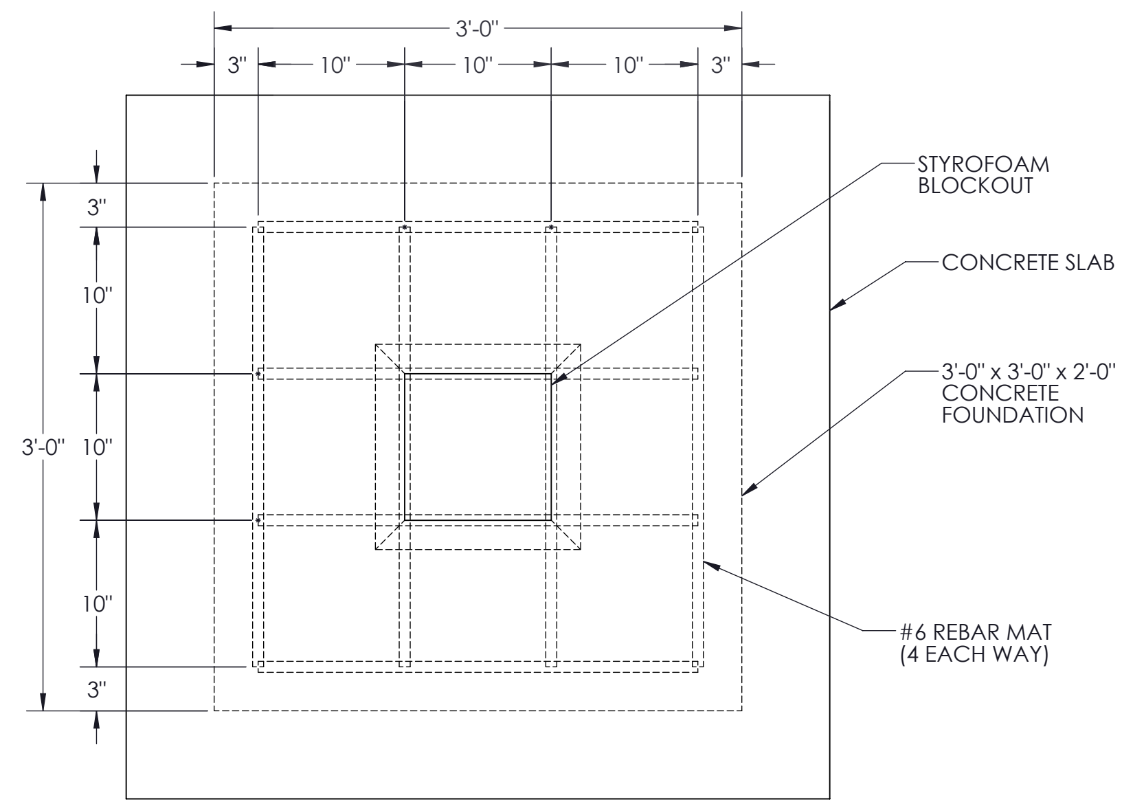
TOP VIEW
