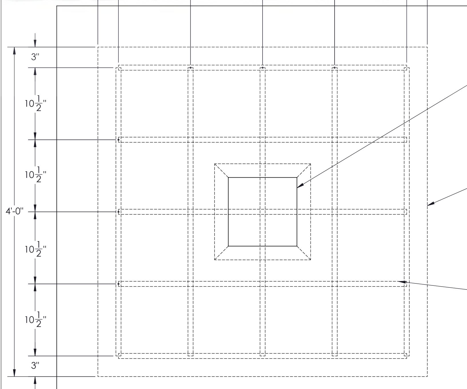
TOP VIEW
