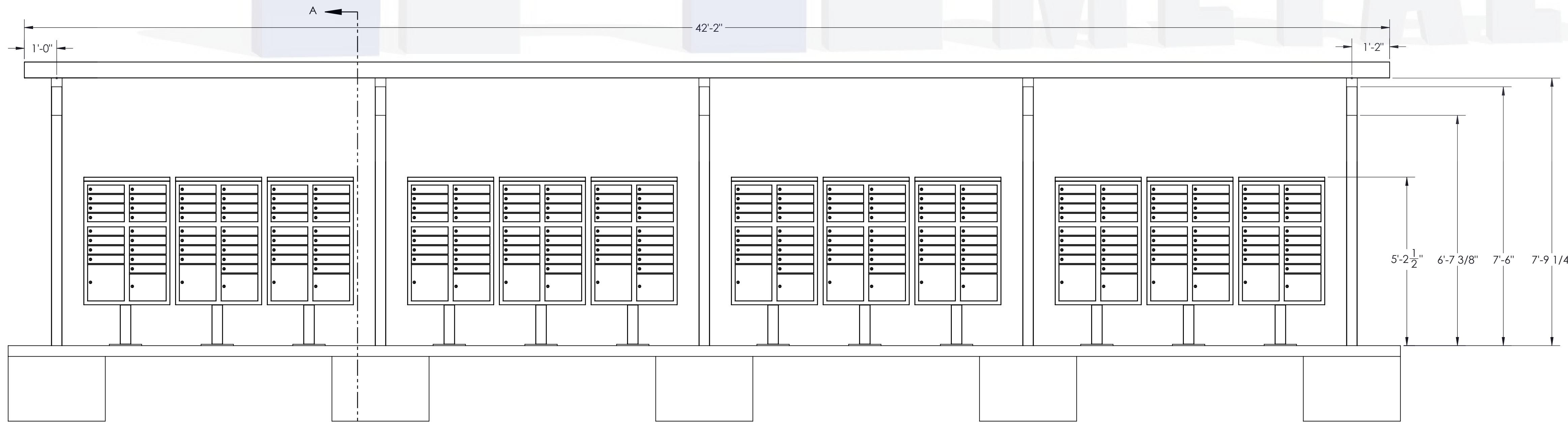
ELEVATION VIEW
