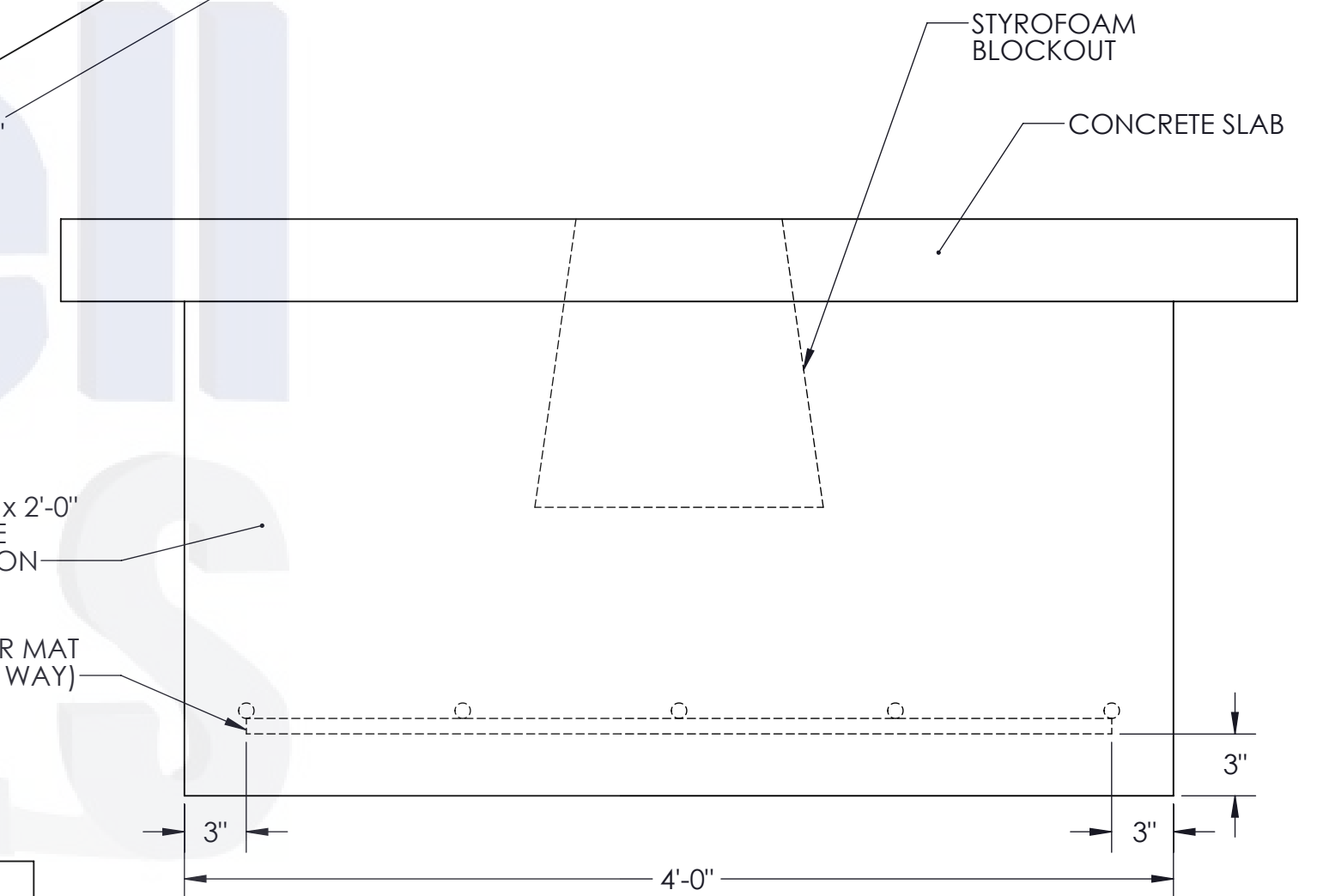
SIDE VIEW
