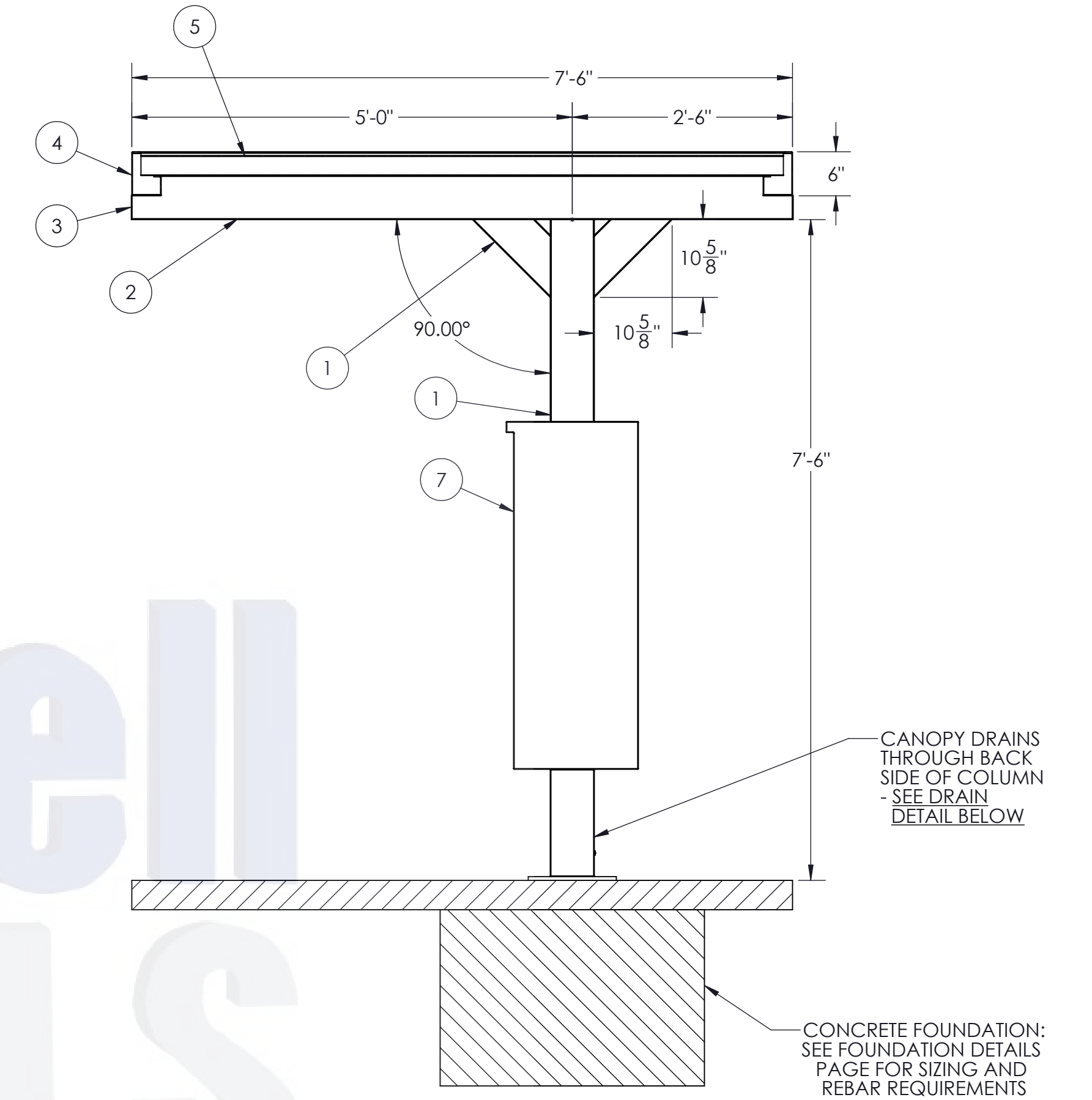
SECTION A-A SCALE 1:16 SECTION VIEW
