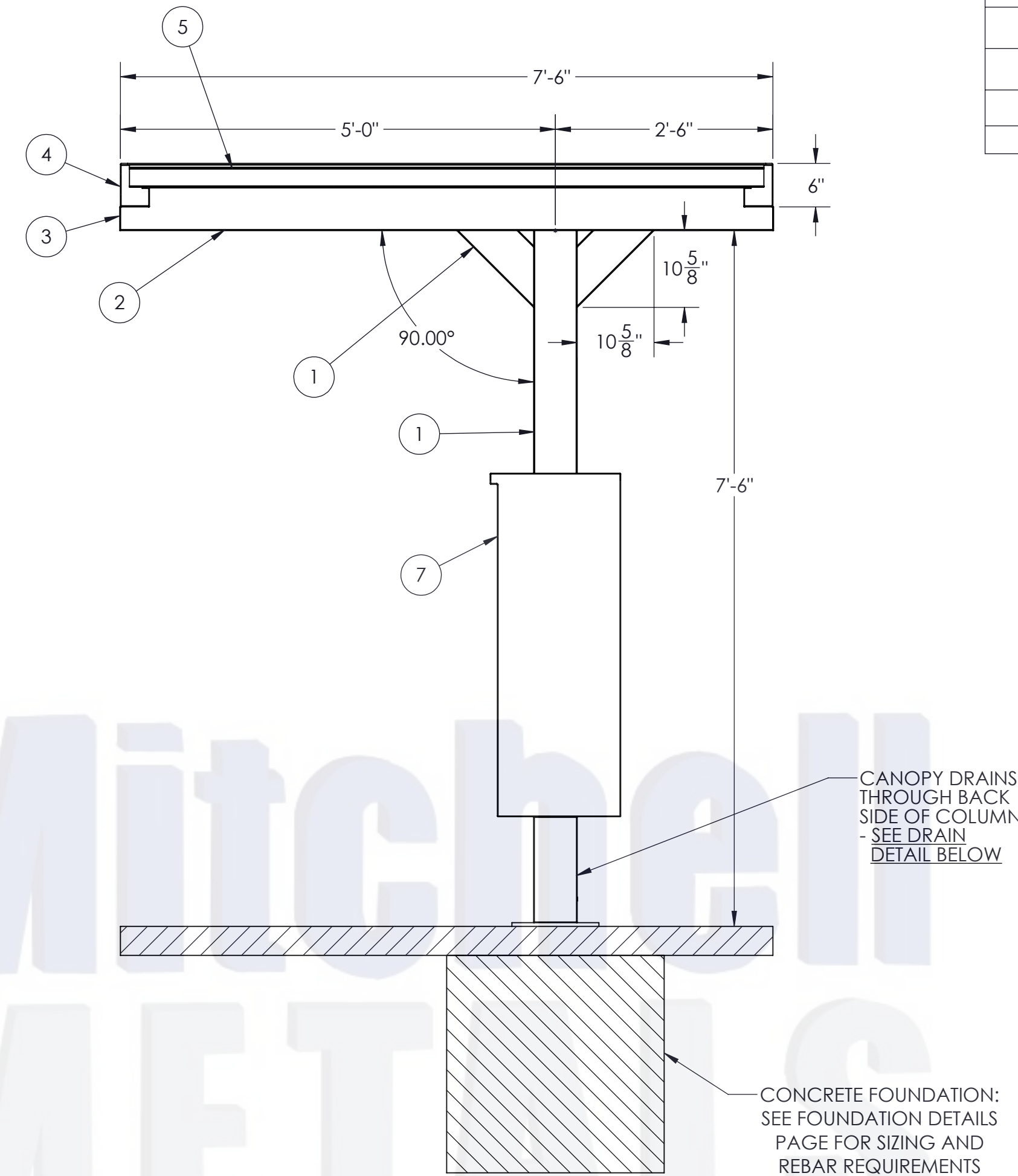
SECTION VIEW
