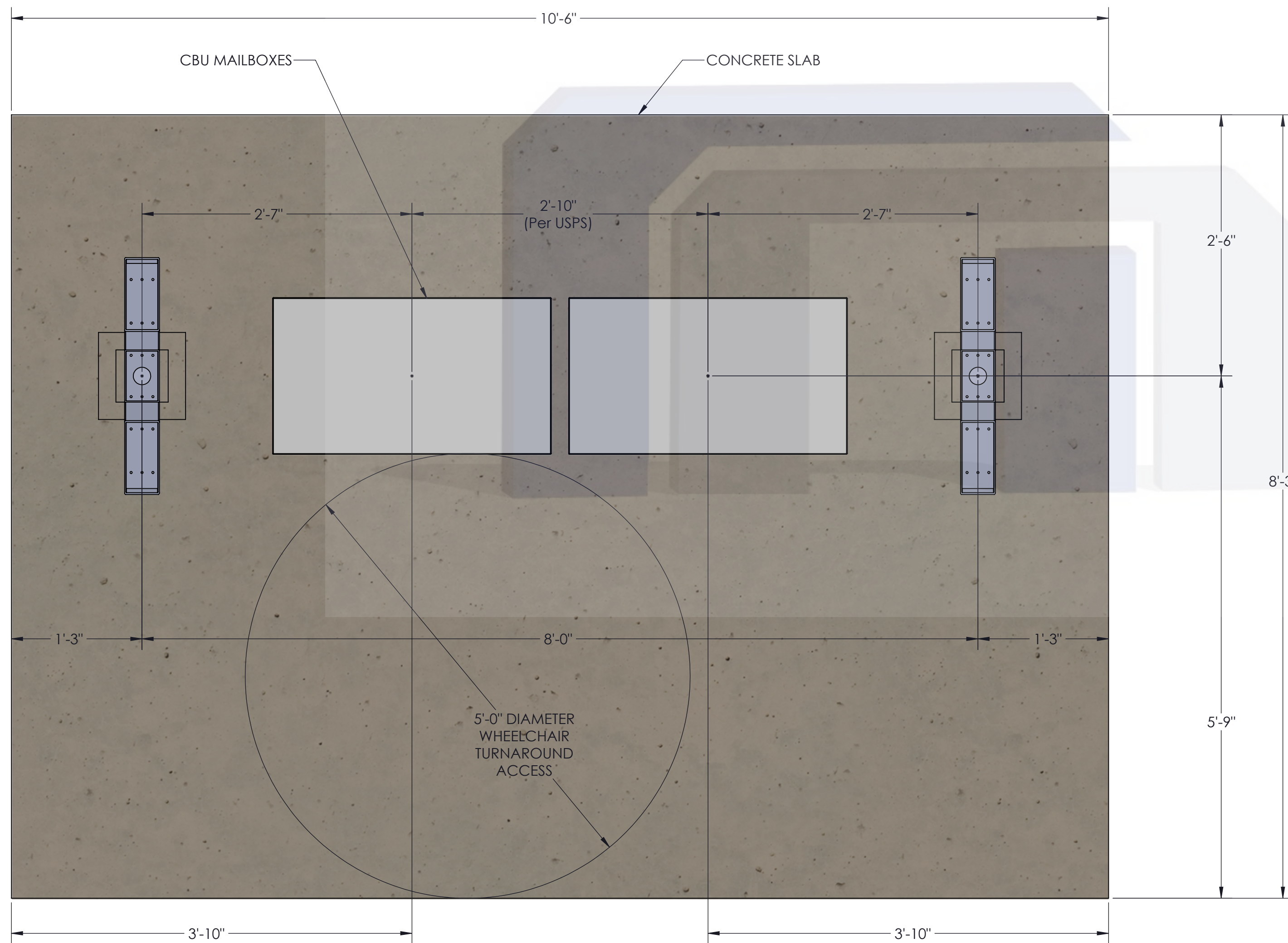
TOP VIEW
