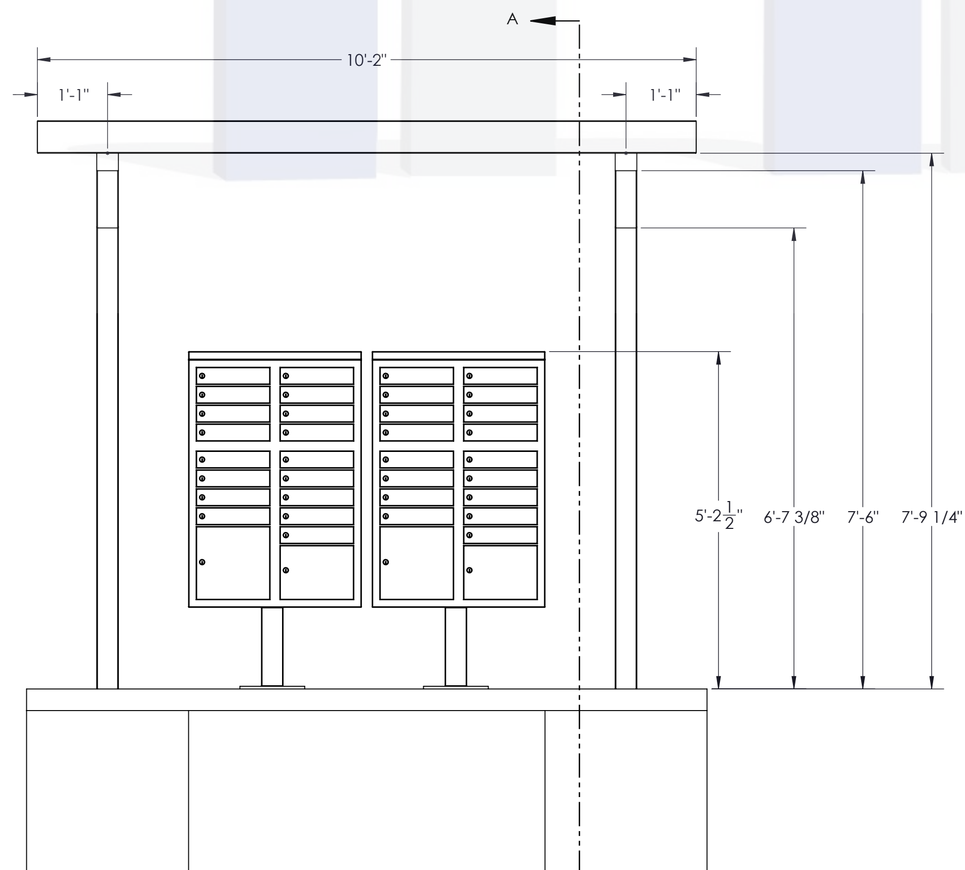
ELEVATION VIEW
