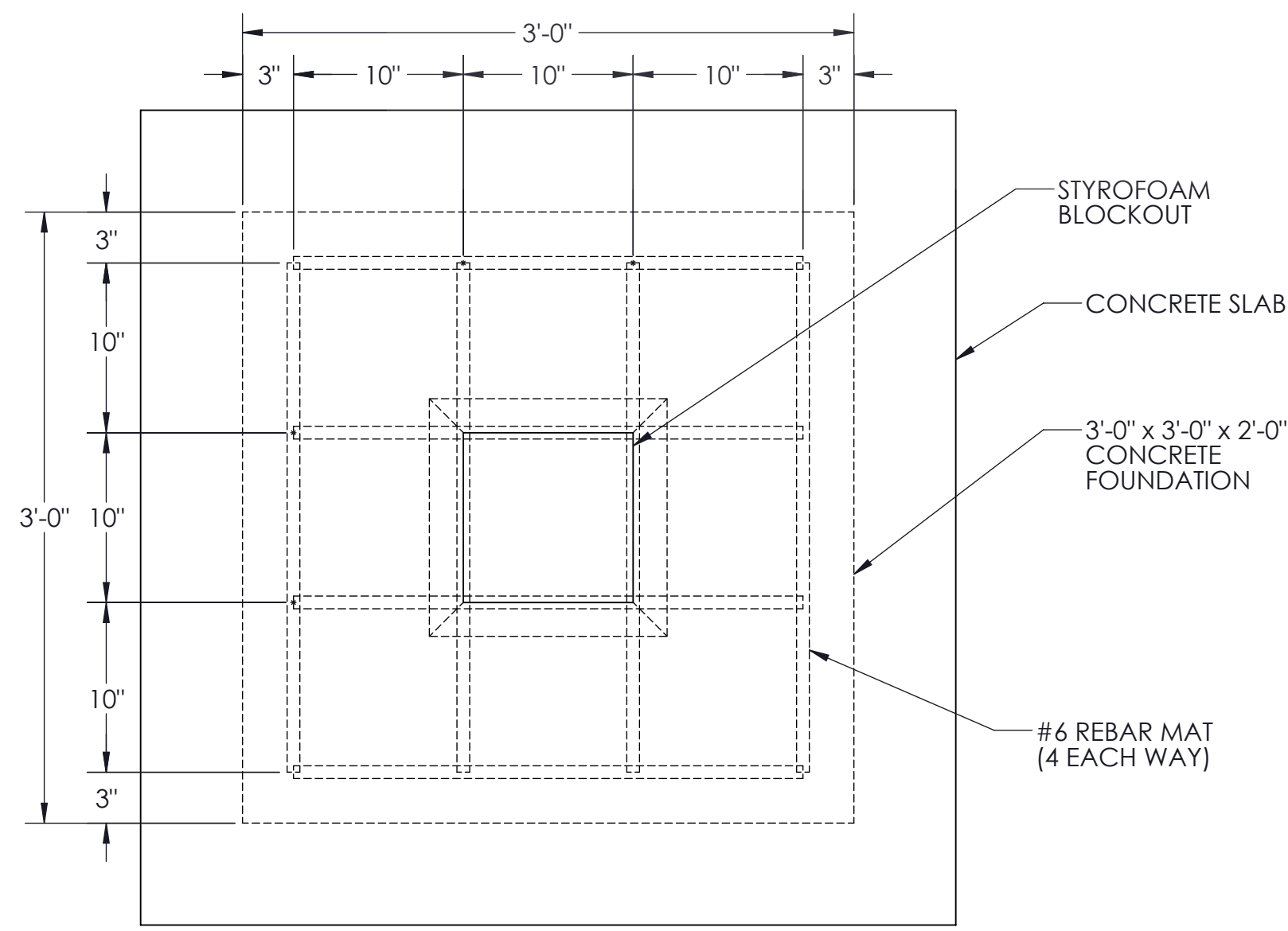
TOP VIEW
