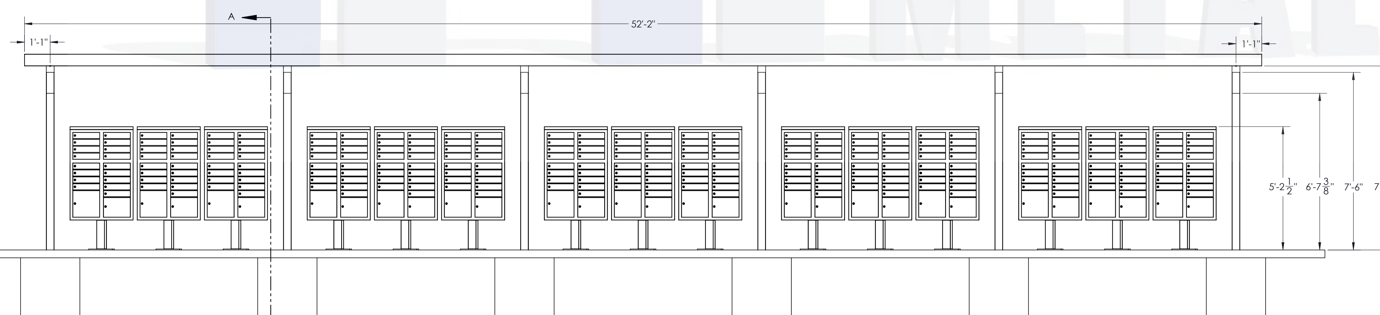
ELEVATION VIEW
