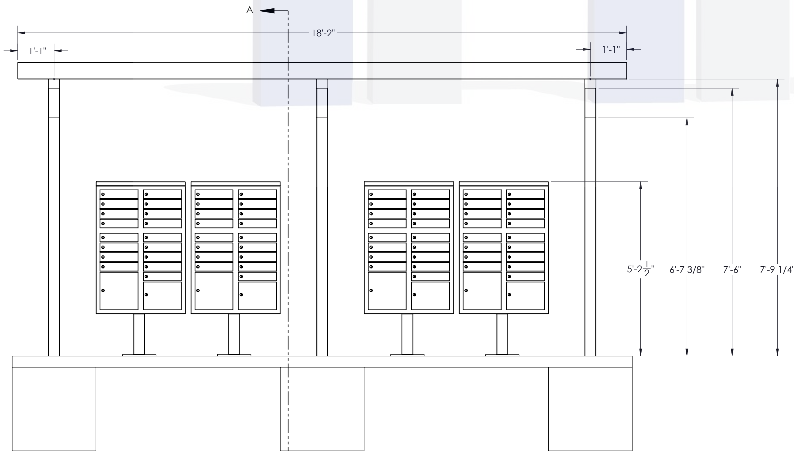
ELEVATION VIEW
