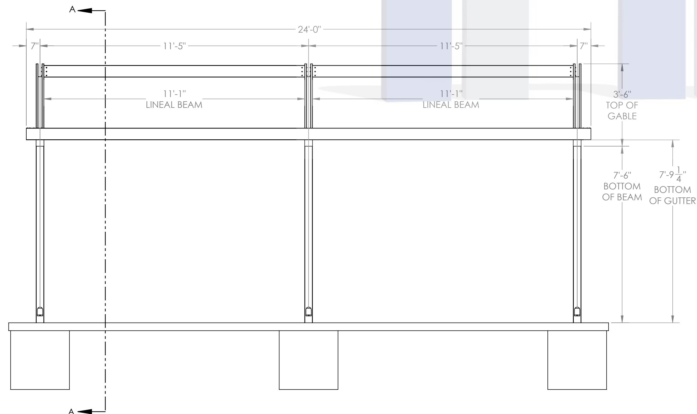
ELEVATION VIEW FRAMING AND GUTTER LAYOUT
