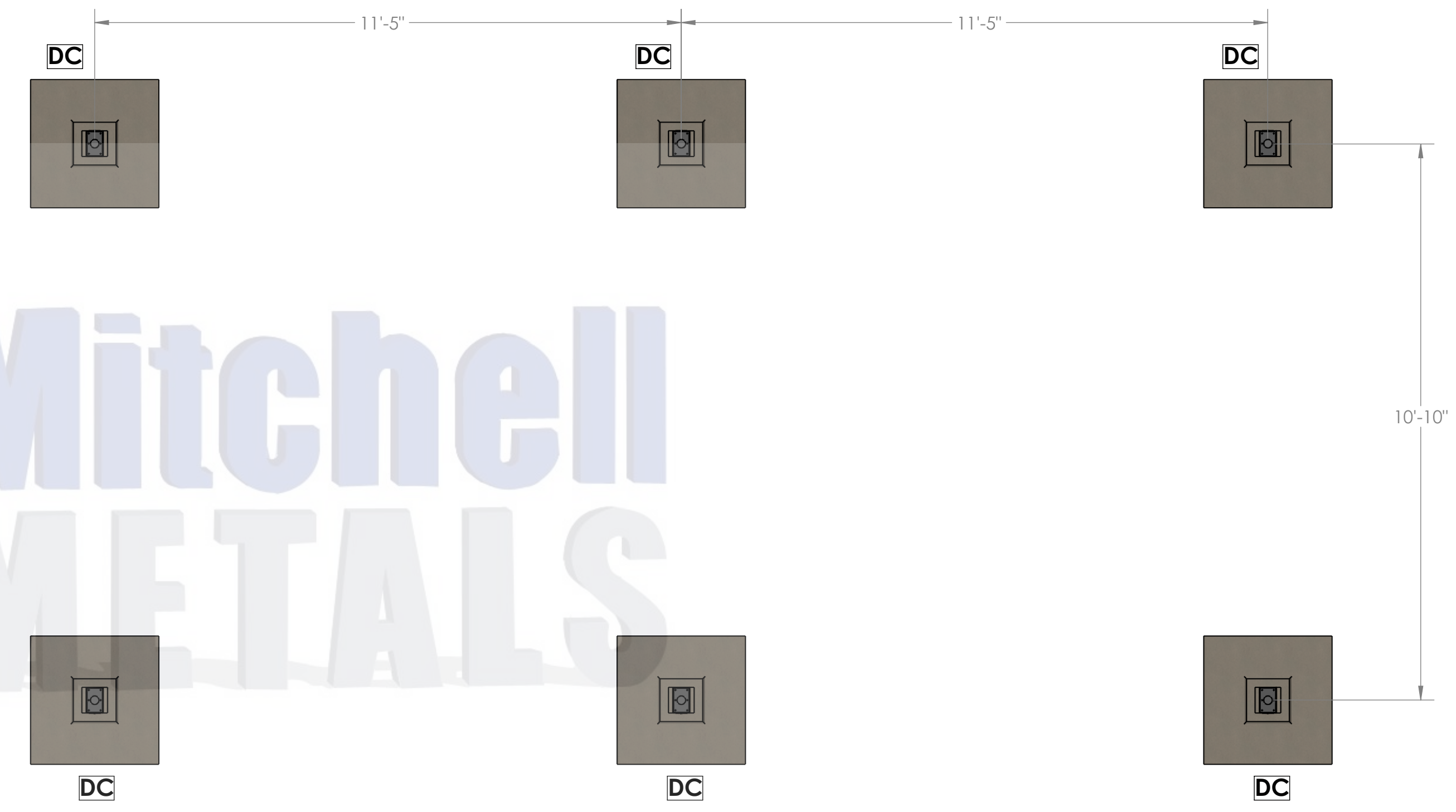
TOP VIEW FOOTING/COLUMN LAYOUT
