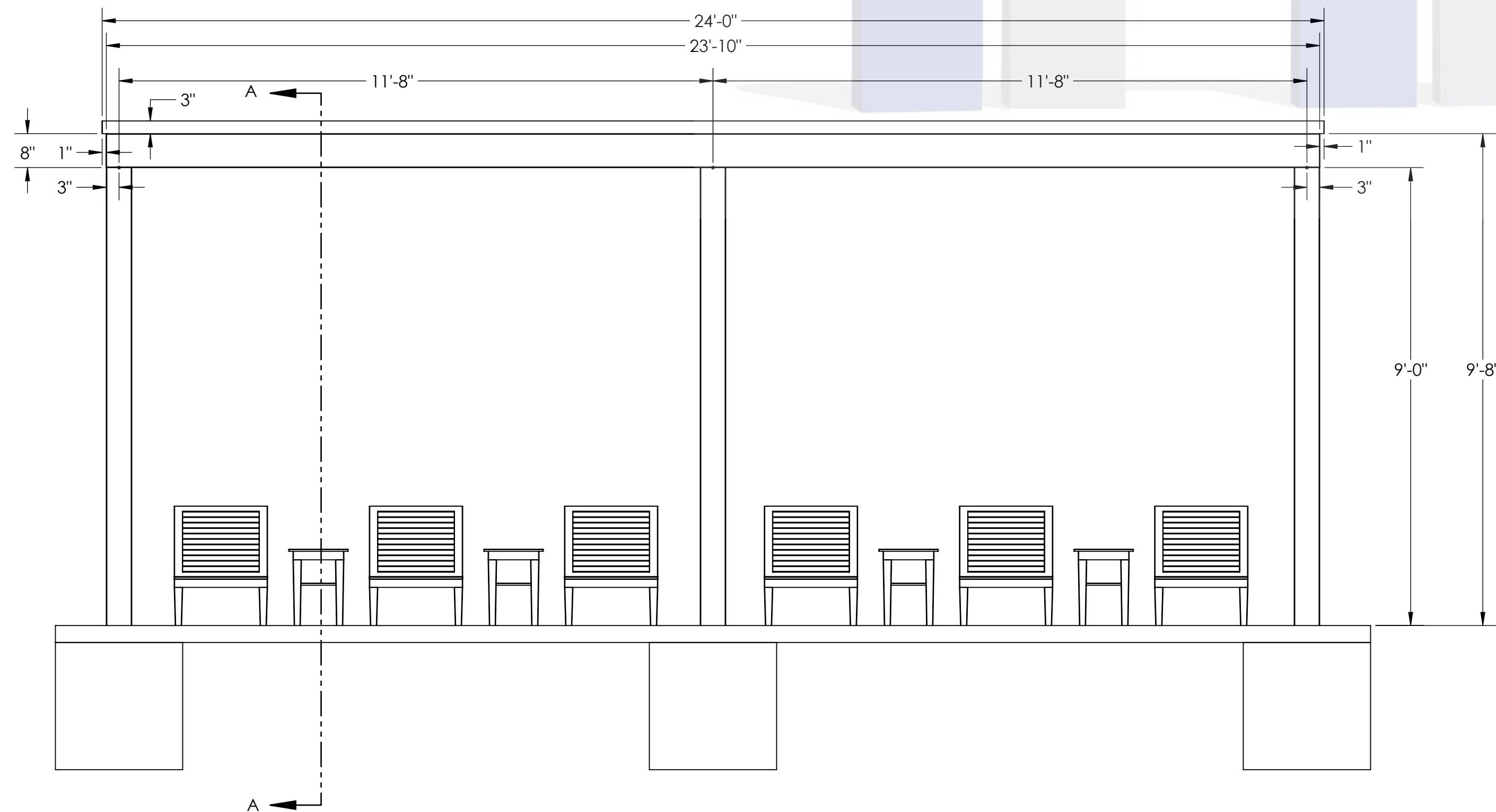
ELEVATION VIEW
