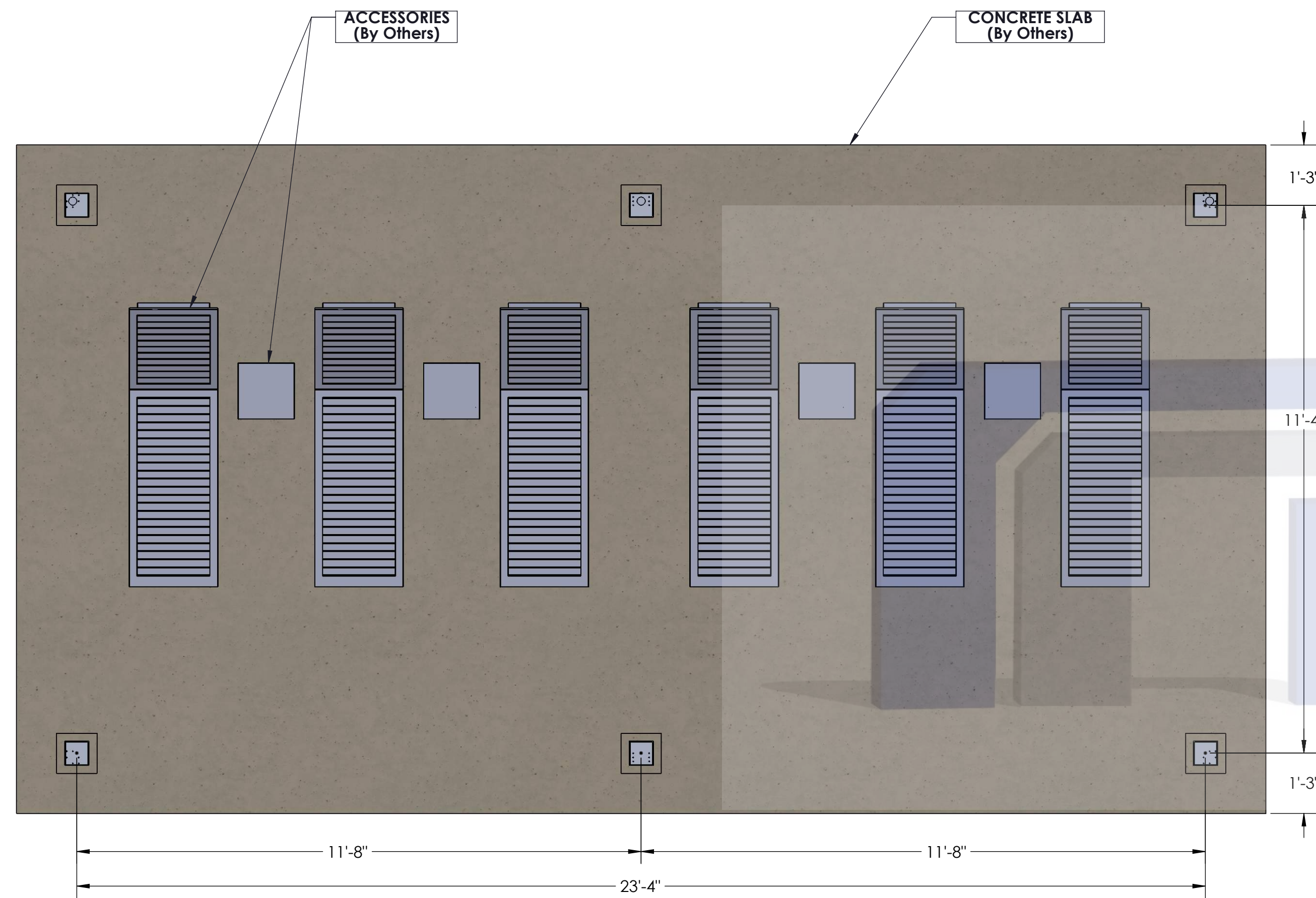
TOP VIEW COLUMN/BENCH/CONCRETE LAYOUT
