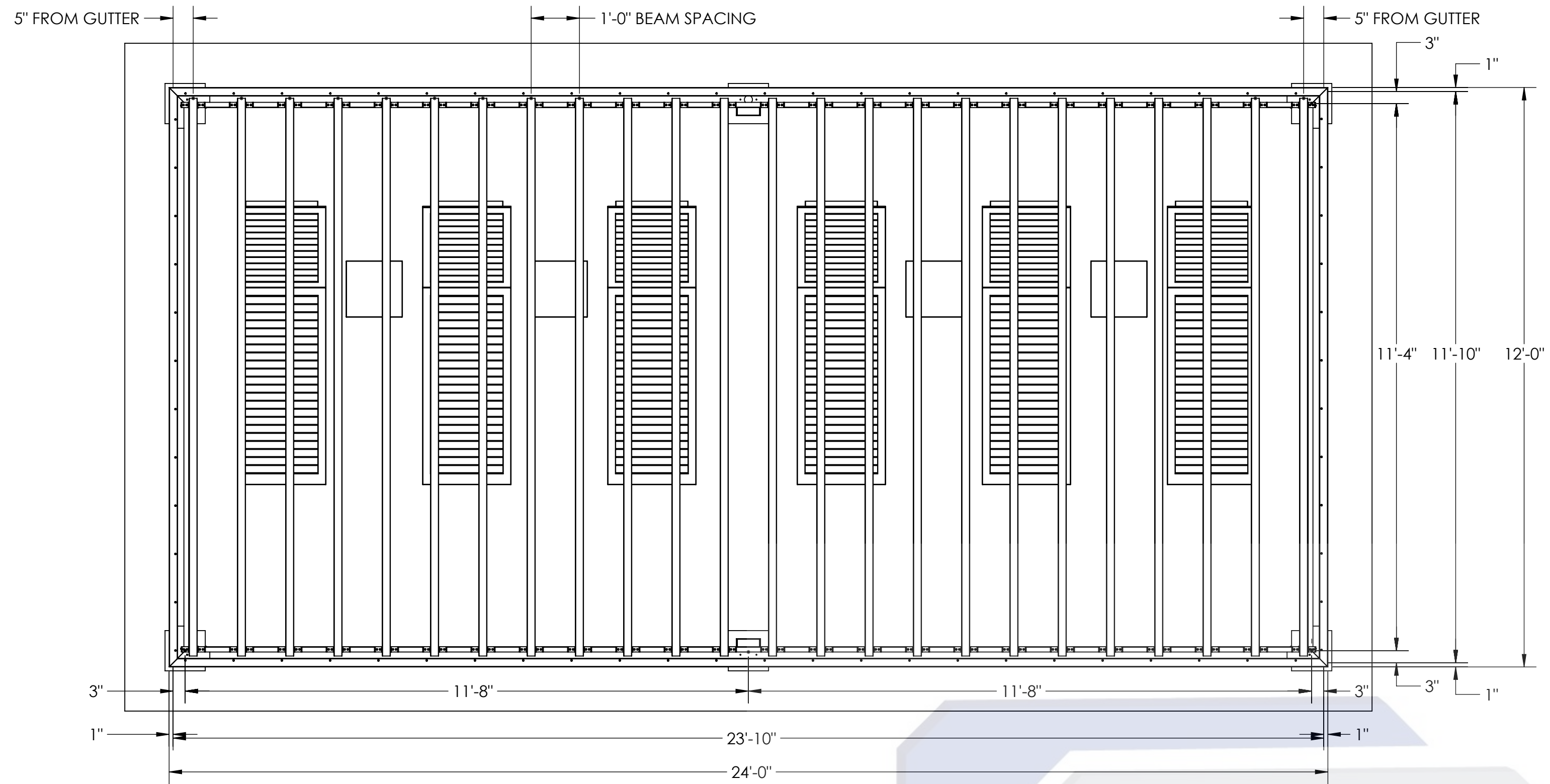
TOP VIEW - NO DECKING FRAMING AND GUTTER LAYOUT
