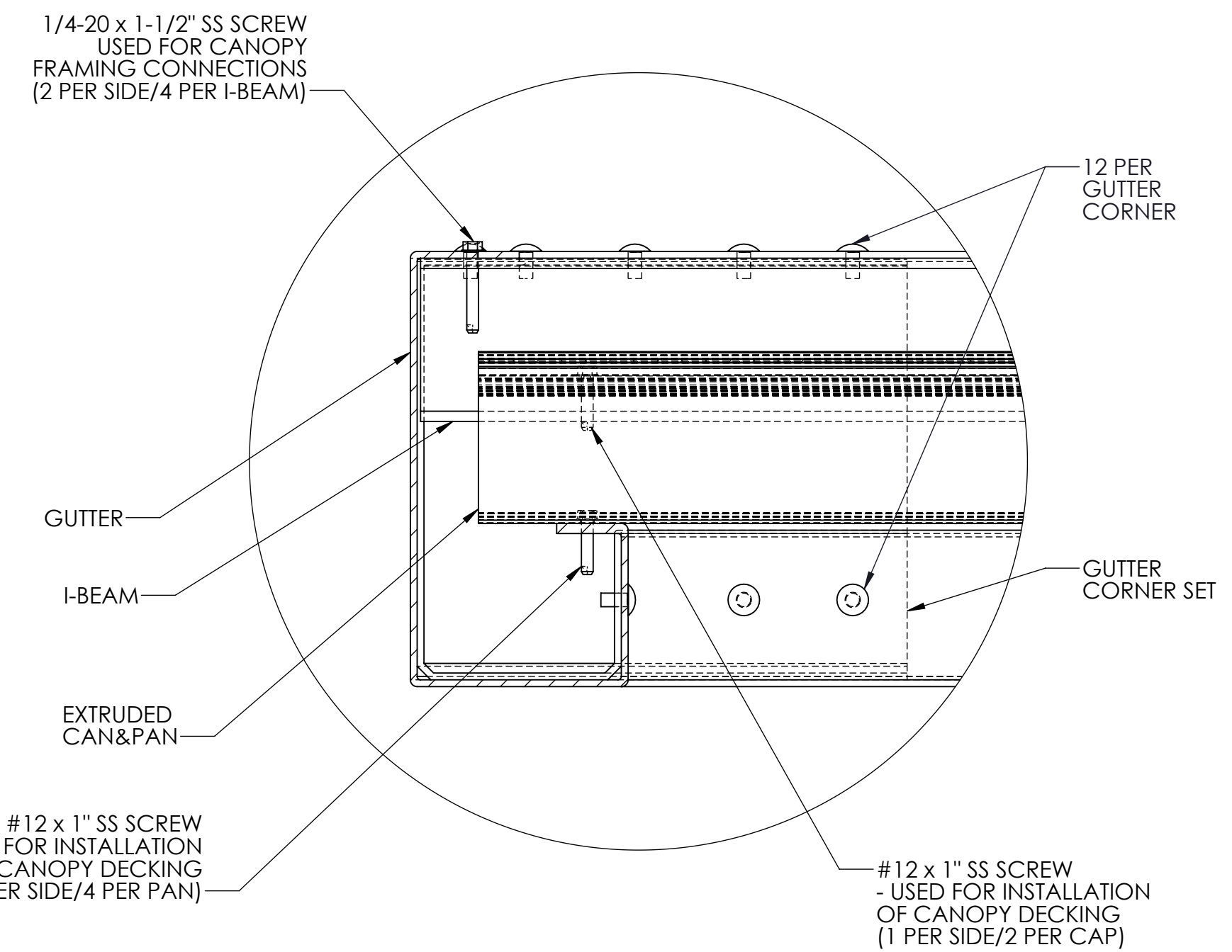
DETAIL D SCALE 1 : 2.5
