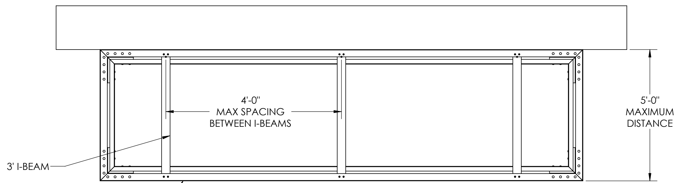
TOP VIEW (NO DECKING)
